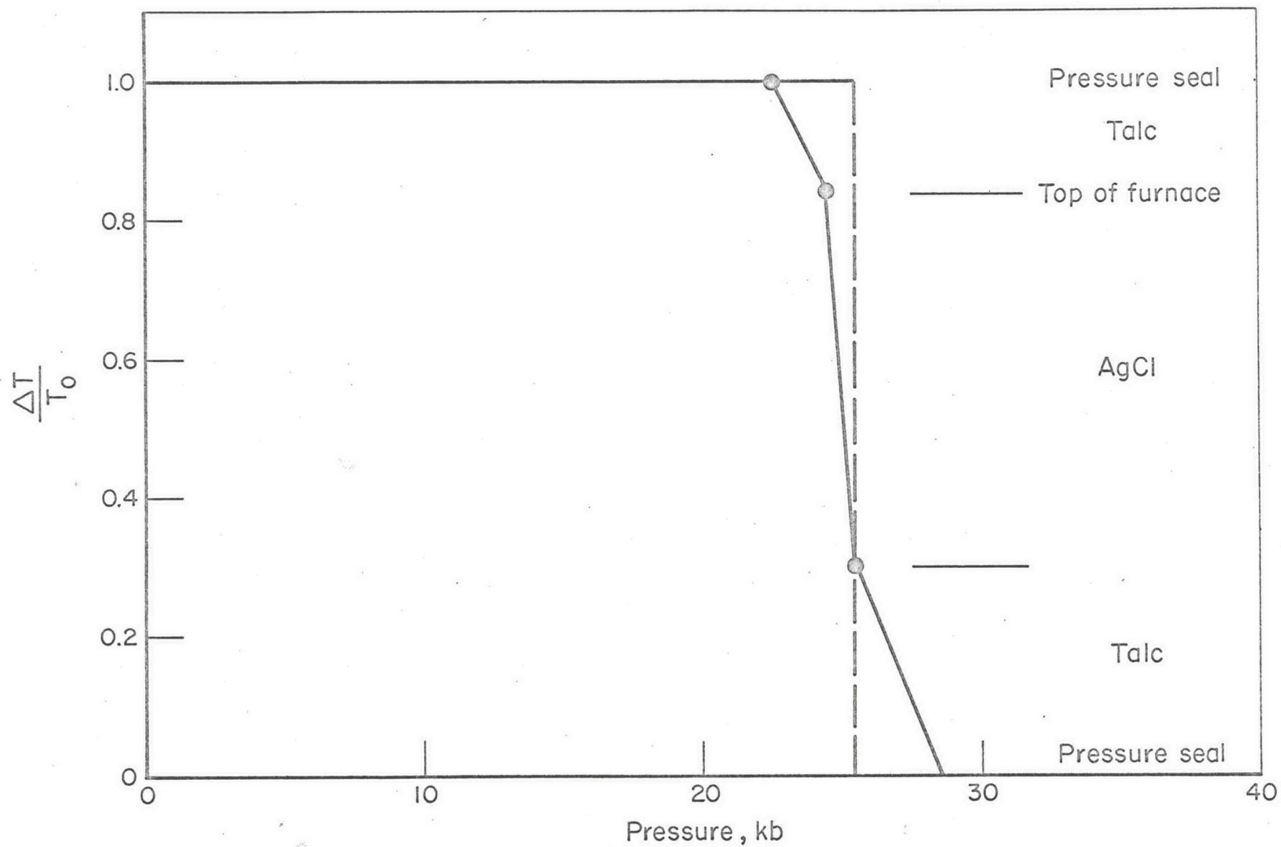
PRESSURE-TEMPERATURE RELATION
